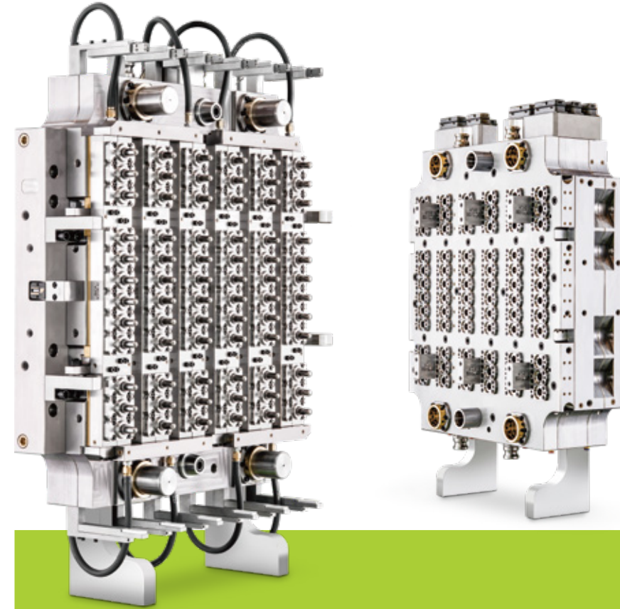
24 CAVITY PREFORM MOLD OF PP IV INFUSION PREFORM WITH HANGER
