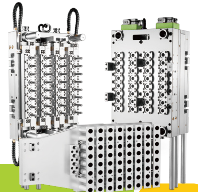
32 CAVITY PREFORM MOLD WITH EOAT PLATE
