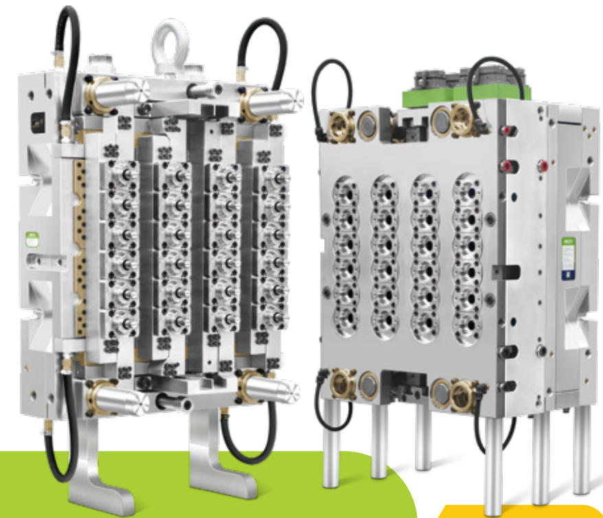
24 CAVITY PREFORM MOLD OF PP IV INFUSION PREFORM WITH HANGER
